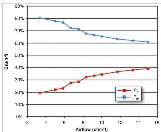
Figure 1: Contribution of air and water to total cooling capacity of an active beam.
