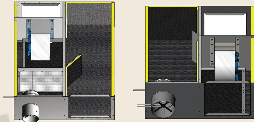
FIGURE 1A (LEFT) Series unit. FIGURE 1B (RIGHT) Parallel unit.
