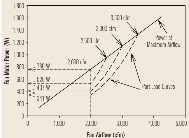
FIGURE 2 Simplified performance evaluation of ECM fan-powered terminal unit energy use.
